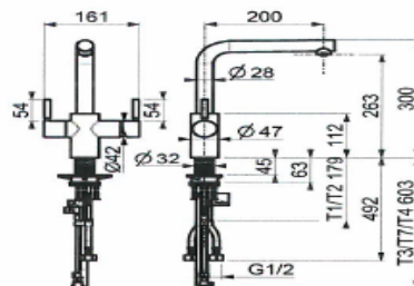
Product dimensions (mm)
